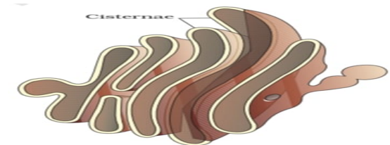
Figure 8.6 Golgi apparatus
