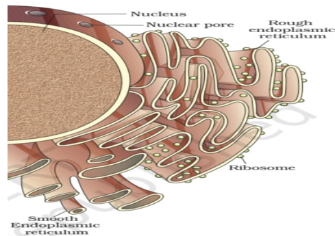
Figure 8.5 Endoplasmic reticulum
